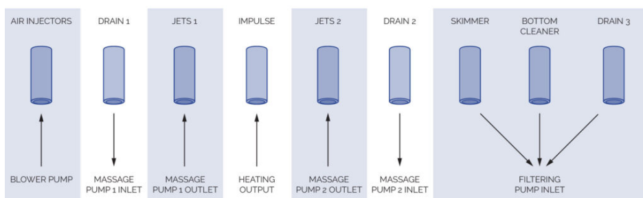
DESCRIPTION OF SPA CONNECTION SYSTEM
