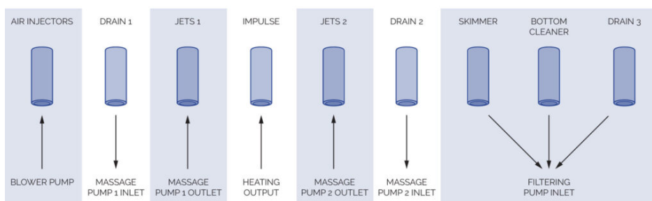
DESCRIPTION OF SPA CONNECTION SYSTEM
