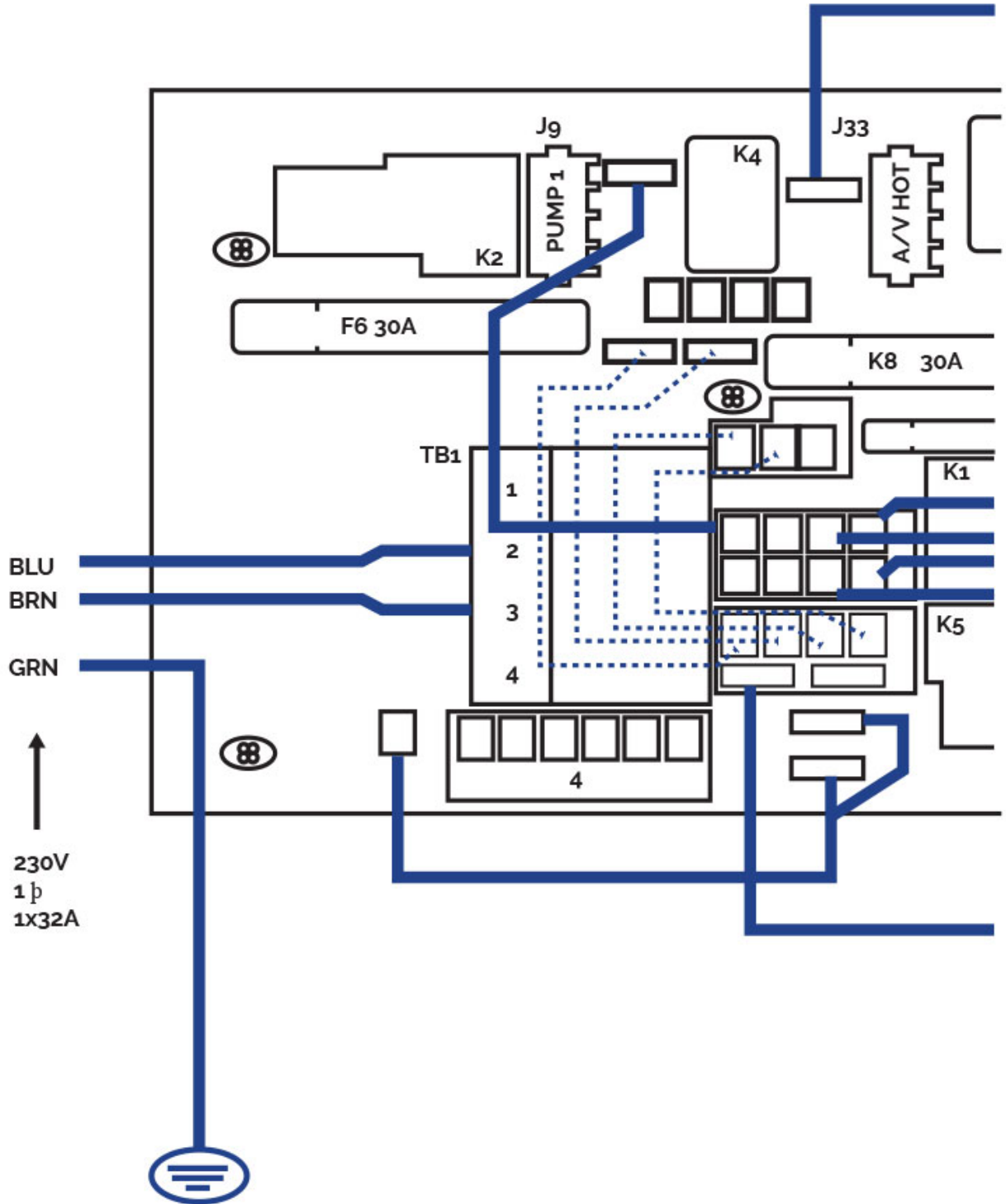
Single line 230V 32A
