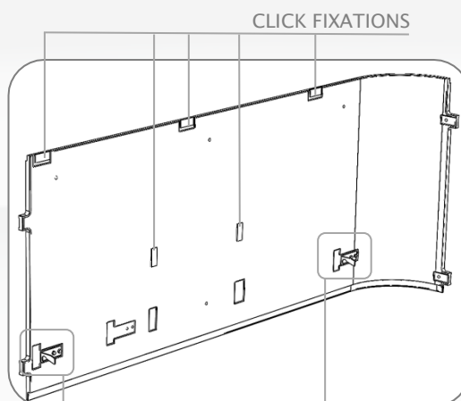
LATERAL SUPPORT HOOK
